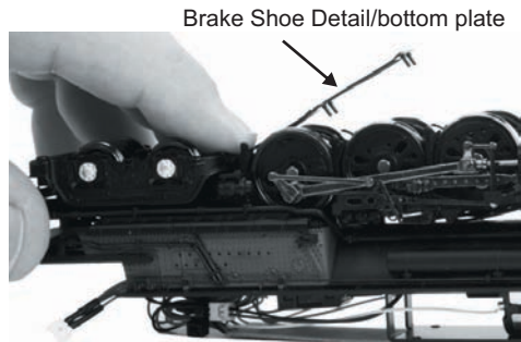
Brake Shoe Detail/bottom plate
